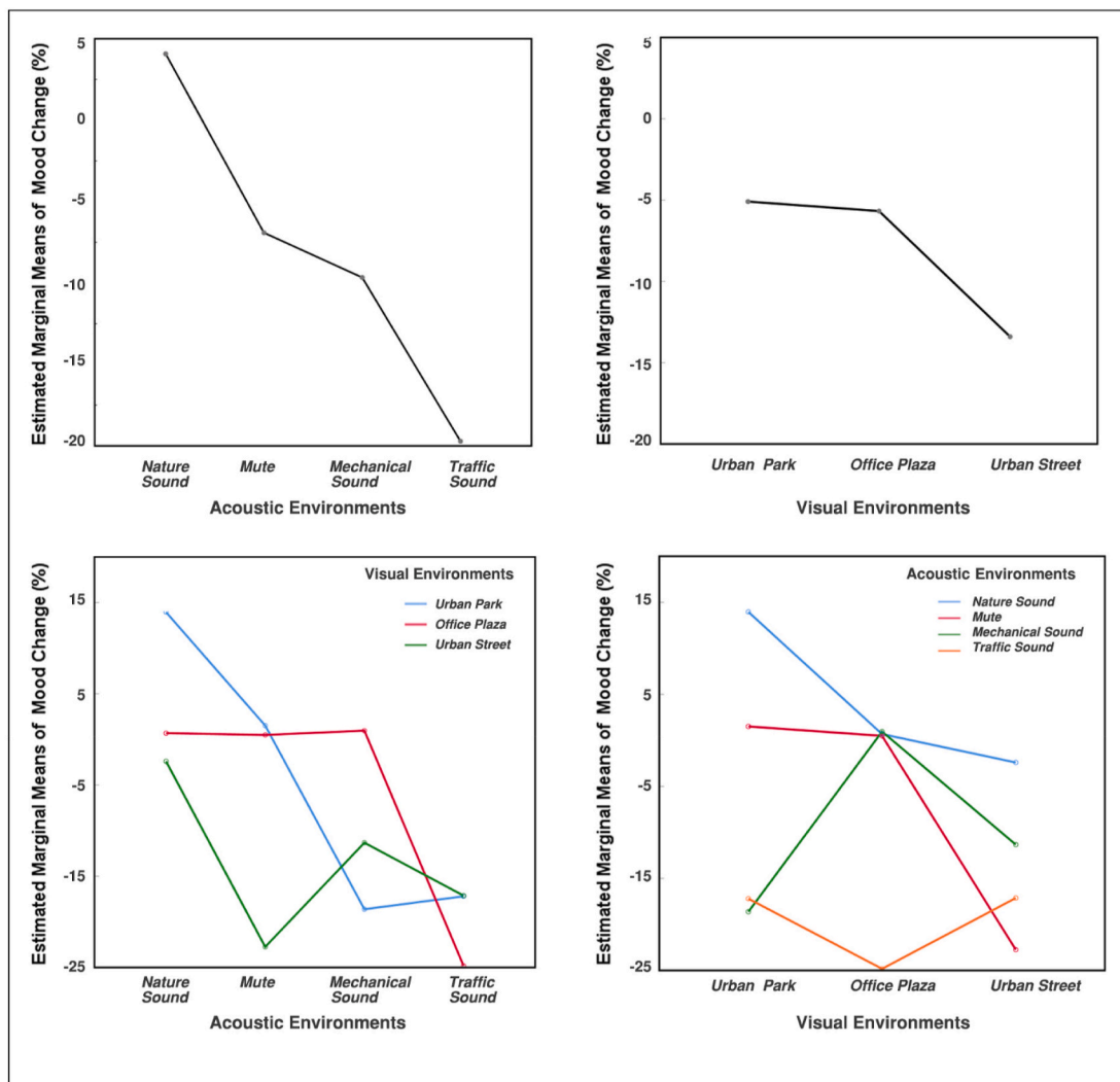
Fig. 4. Plot of two-way analysis of variance (combined data from two experiments). The top row shows the main effects for acoustic and visual environments. The bottom row shows the interactive effects for both environments.
