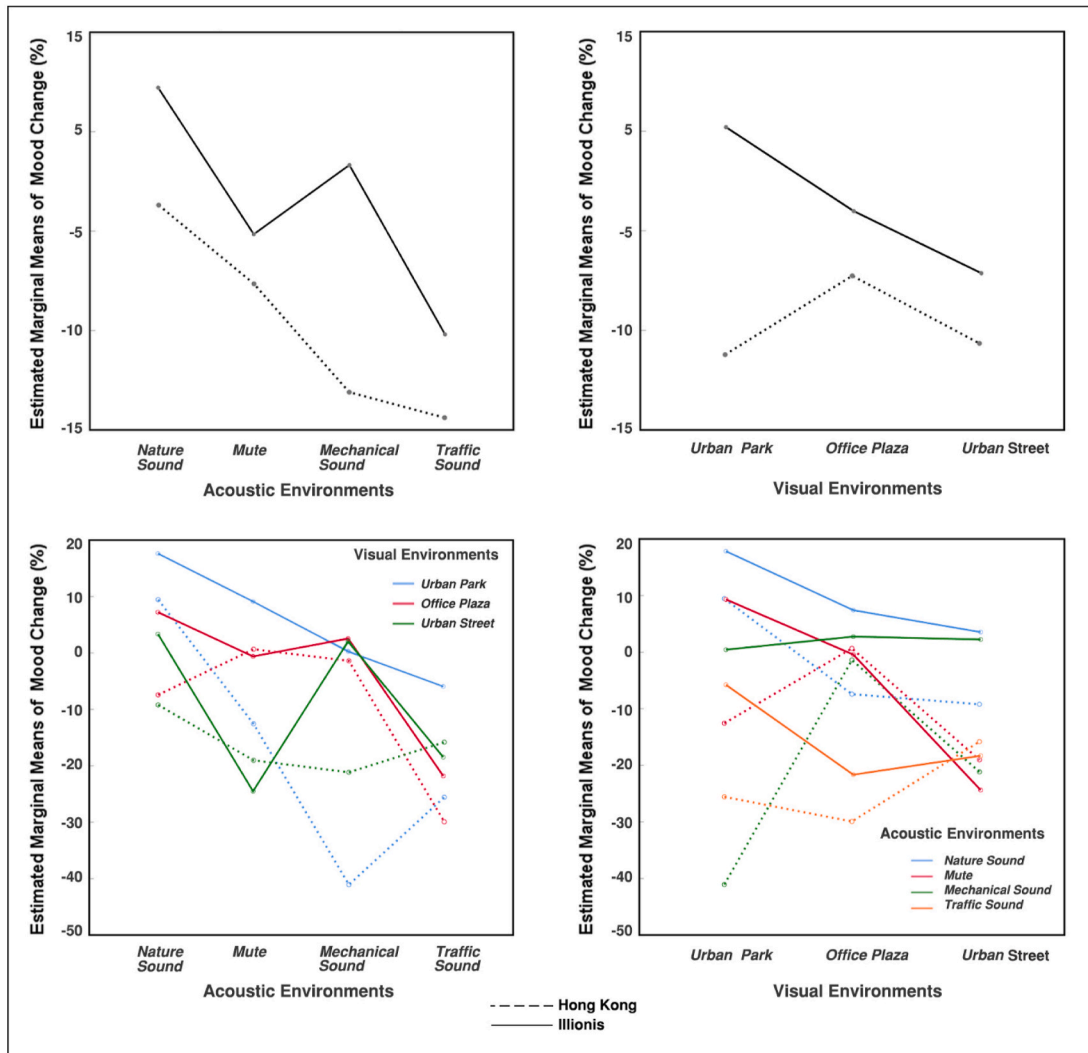
Fig. 5. Plot of two-way analysis of variance (for Illinois and Hong Kong, respectively). The top row shows the main effects for acoustic and visual environments. The bottom row shows the interactive effects for both environments.
